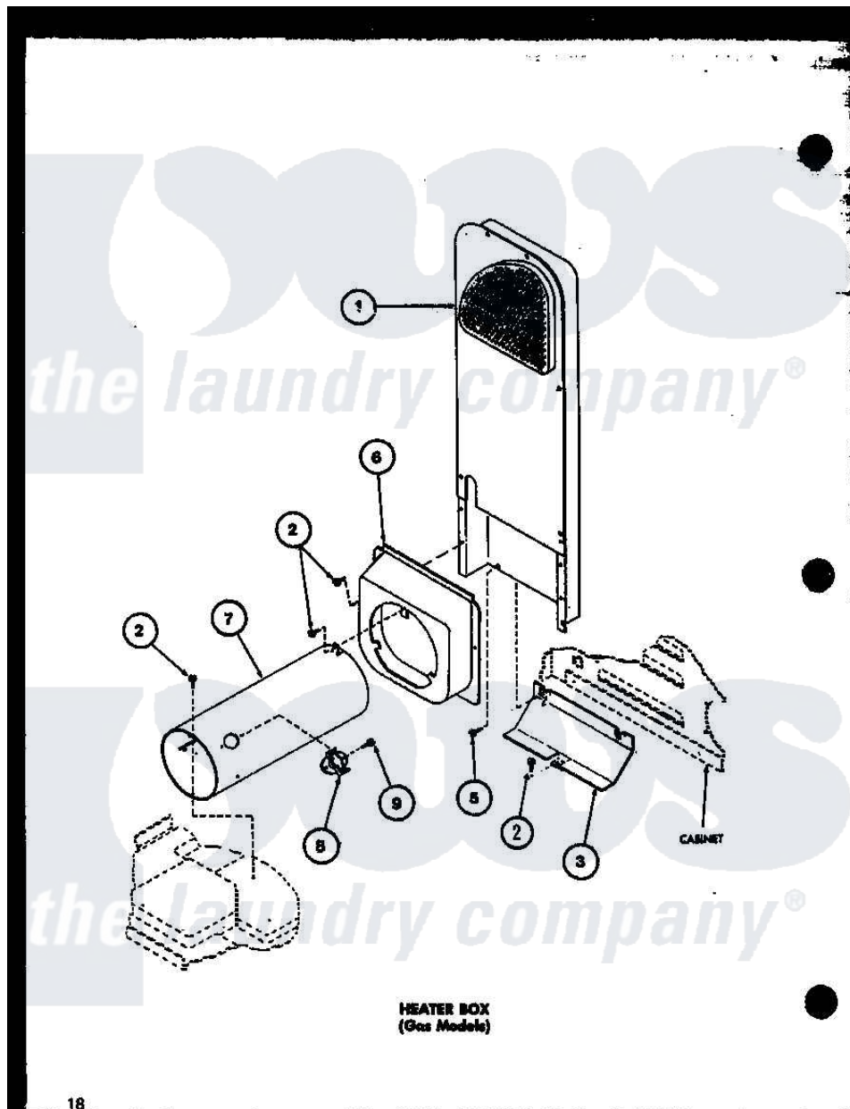
Amana Residential Amana LG3812W (BOM: P1122701W W) Dryer Parts Parts Diagram 04 - HEATER BOX (GAS MODELS)
