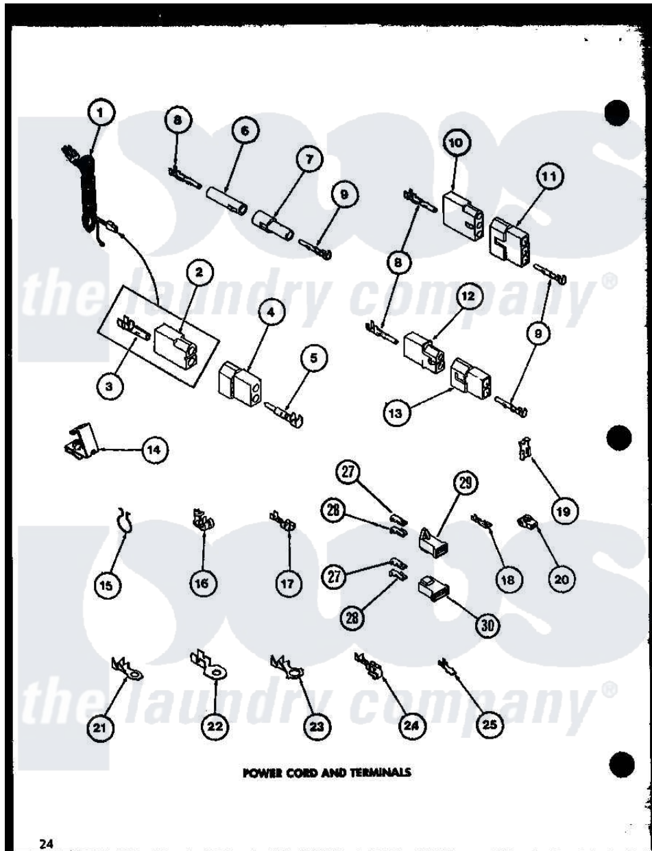
Amana Residential Amana LG3912W (BOM: P1122703W W) Dryer Parts Parts Diagram 08 - POWER CORD AND TERMINALS
