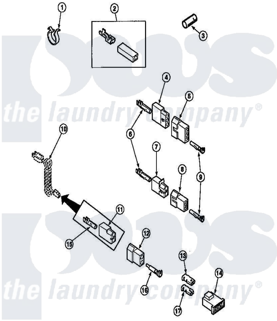
Amana Residential Amana LG8109W2 (BOM: PLG8109W2) Dryer Parts Parts Diagram 20 - TERMINALS Click on the part number to view part
