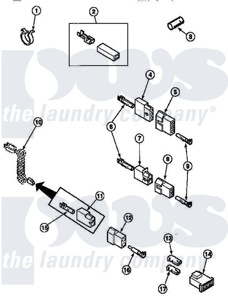
Amana Residential Amana LG8219L2 (BOM: PLG8219L2) Dryer Parts Parts Diagram 20 - TERMINALS Click on the part number to view part
