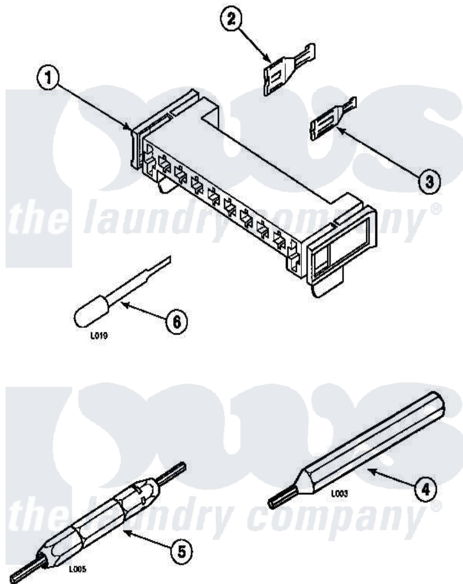
Amana Residential Amana LG8219W2 (BOM: PLG8219W2) Dryer Parts Diagram 16 - Page 21 Click on the part number to view part
