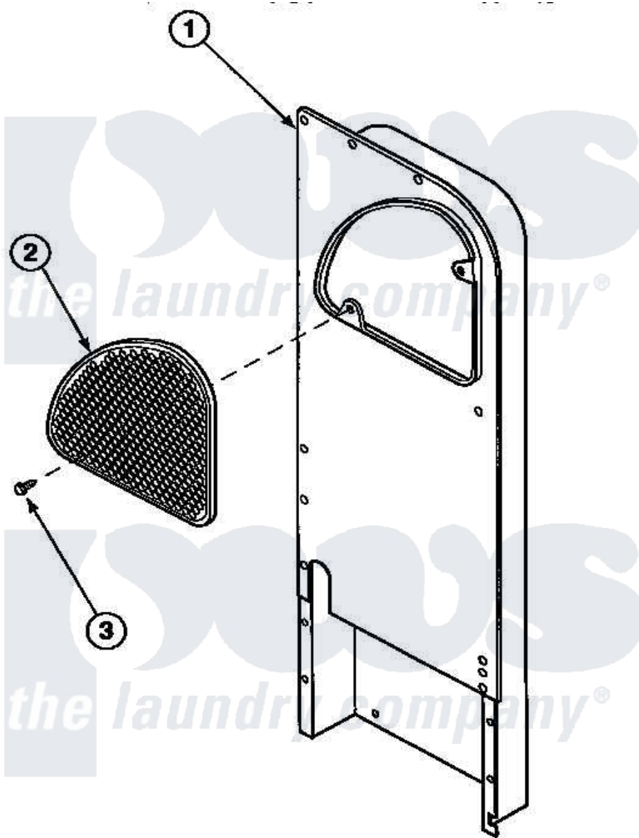
Amana Residential Amana LG8409L2 (BOM: PLG8409L2) Dryer Parts Parts Diagram 12 - HEATER BOX ASSY REPLACEMENT
