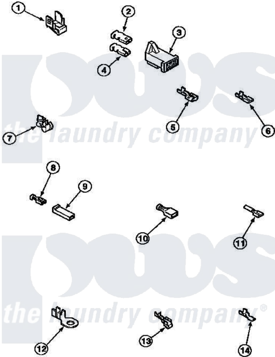
Amana Residential Amana LG8459L2 (BOM: PLG8459L2) Dryer Parts Parts Diagram 21 - TERMINALS Click on the part number to view part
