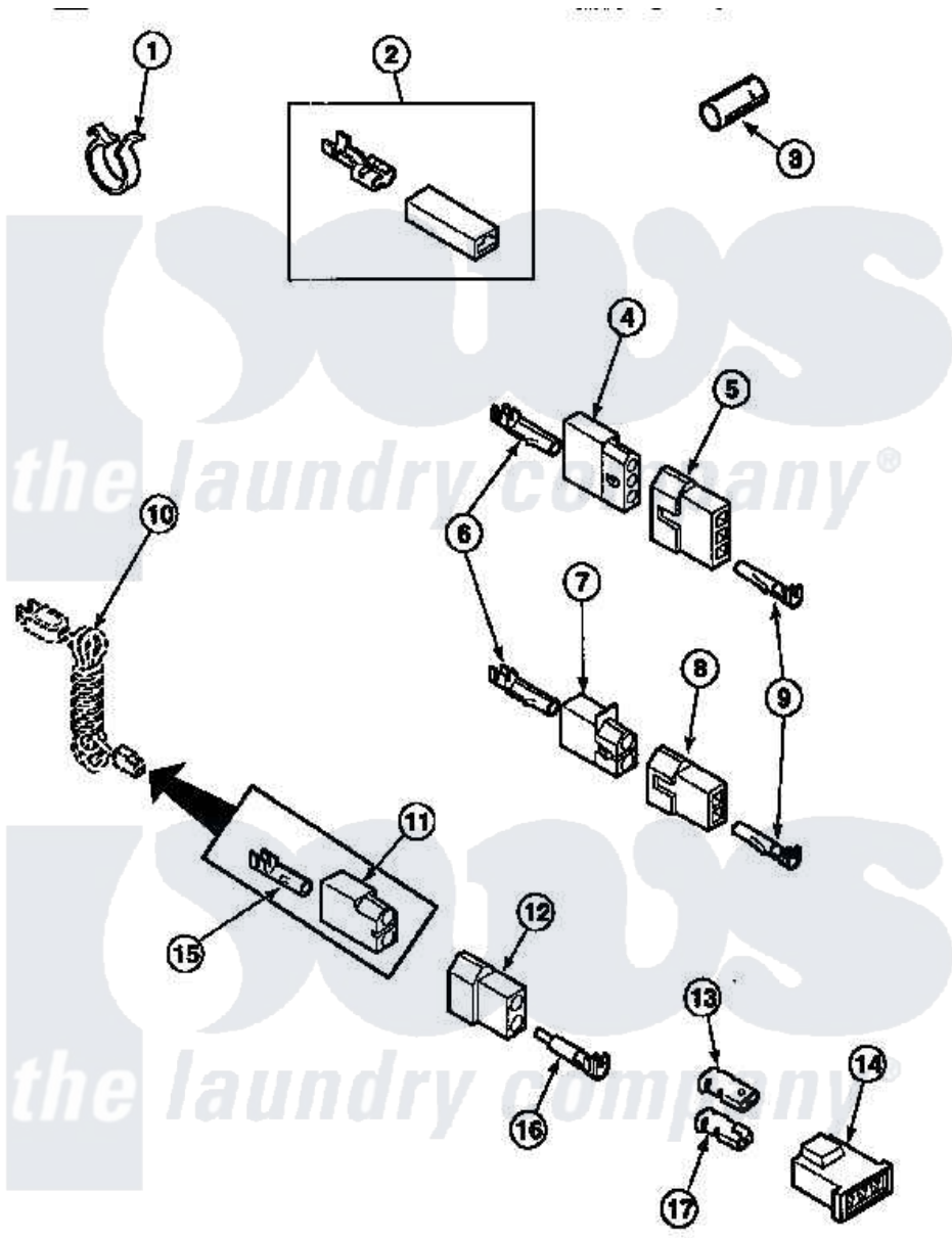
Amana Residential Amana LG8609L2 (BOM: PLG8609L2) Dryer Parts Parts Diagram 20 - TERMINALS Click on the part number to view part
