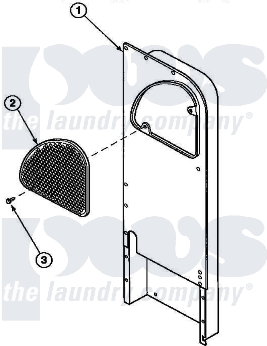
Amana Residential Amana LG9209L2 (BOM: PLG9209L2) Dryer Parts Parts Diagram 12 - HEATER BOX ASSY REPLACEMENT
