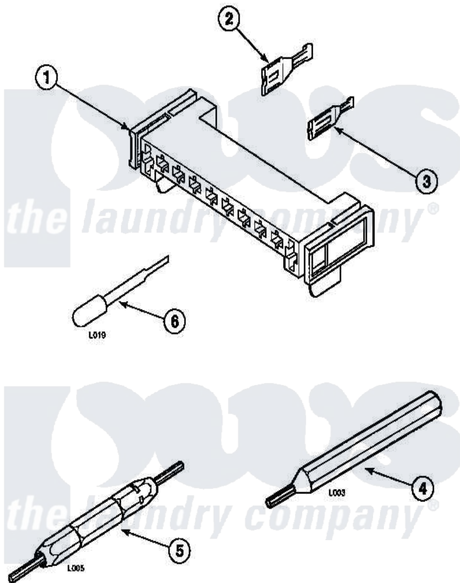
Amana Residential Amana LG9209L2 (BOM: PLG9209L2) Dryer Parts Parts Diagram 16 - Page 21
