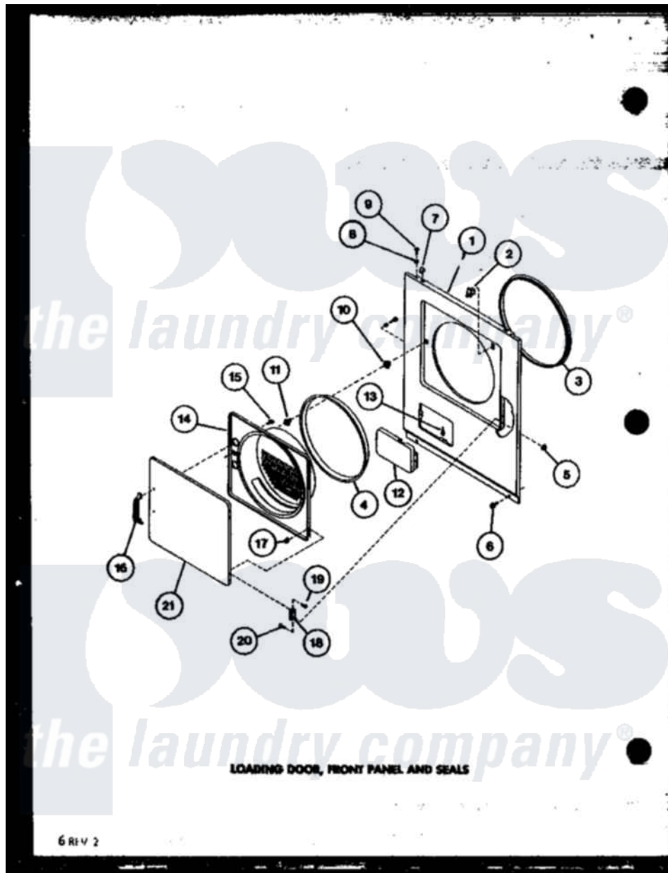
Amana Residential Amana LGD251 (BOM: P7762208W W) Washer Parts Parts Diagram 05 - LOADING DOOR Click on the part number to view part
