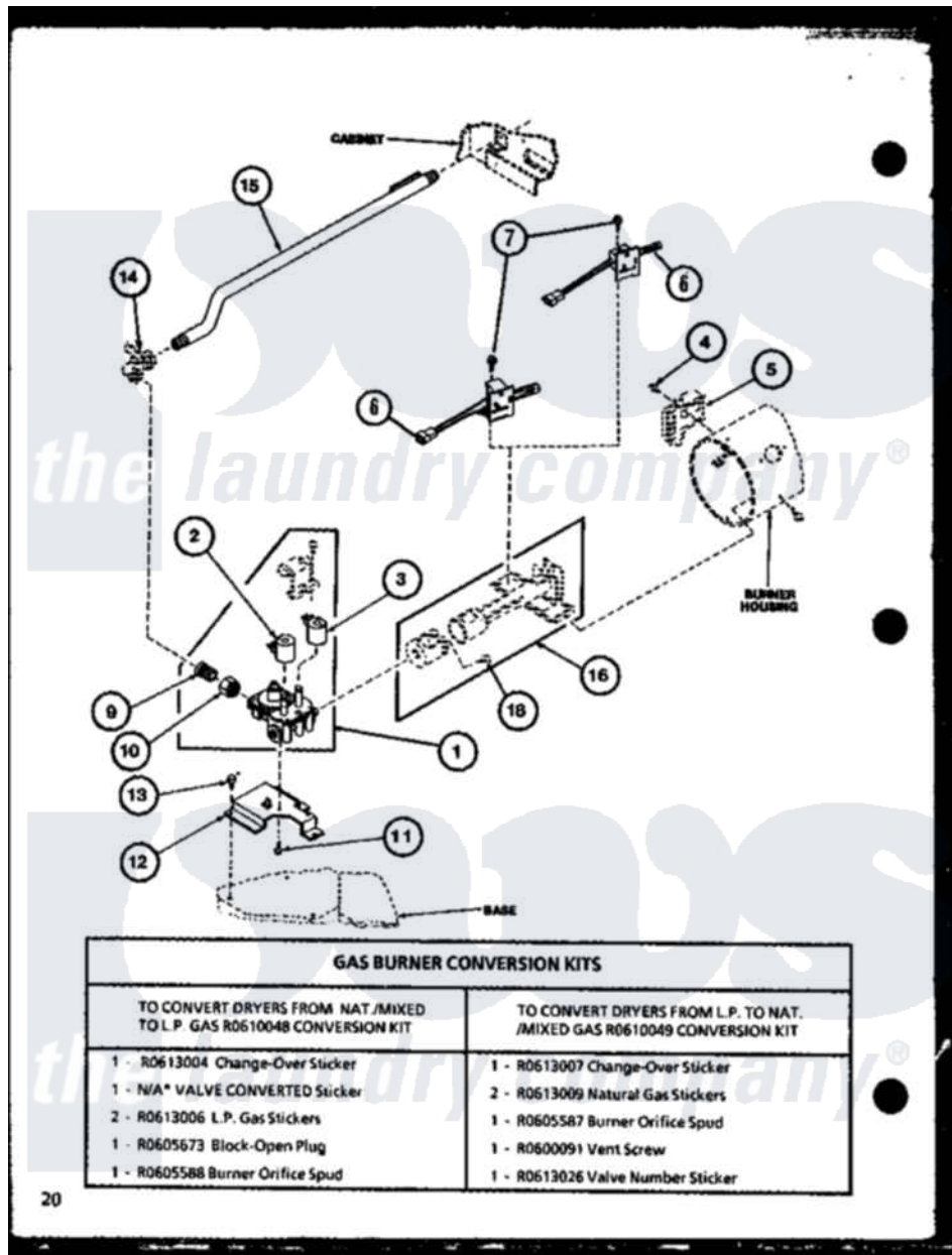
Amana Residential Amana LGD312 (BOM: P776222W W) Dryer Parts Parts Diagram 07 - Page 9 Click on the part number to view part
