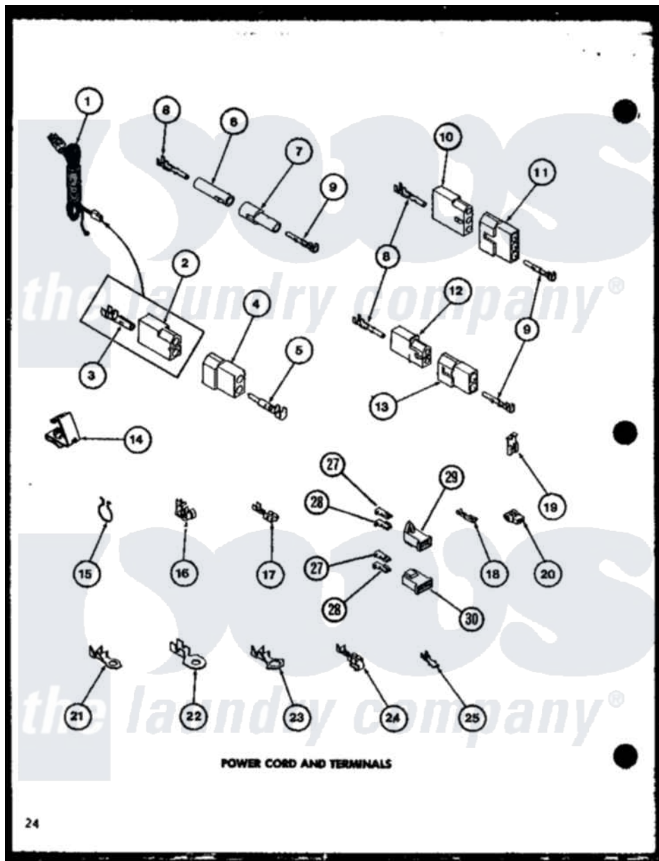
Amana Residential Amana LGD312 (BOM: P776222W W) Dryer Parts Parts Diagram 08 - POWER CORD AND TERMINALS
