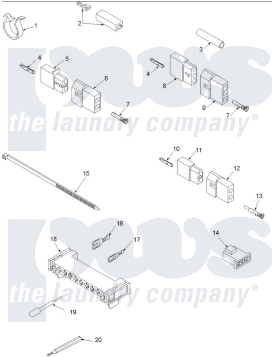
Amana Residential Amana LGD32AW (BOM: PLGD32AW) Dryer Parts Parts Diagram 10 - TERMINALS AND MOTOR CONNECTION BLOCK
