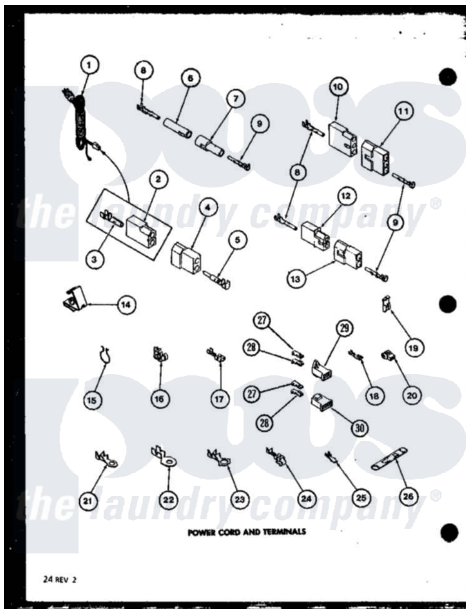
Amana Residential Amana LGD451 (BOM: P7762210W W) Washer Parts Parts Diagram 08 - POWER CORD AND TERMINALS
