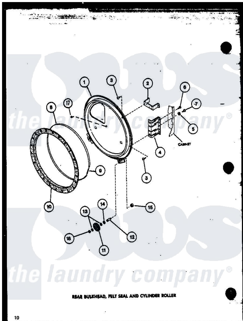
Amana Residential Amana LGD512 (BOM: P7762224W W) Dryer Parts Parts Diagram 09 - REAR BULKHEAD Click on the part number to view part
