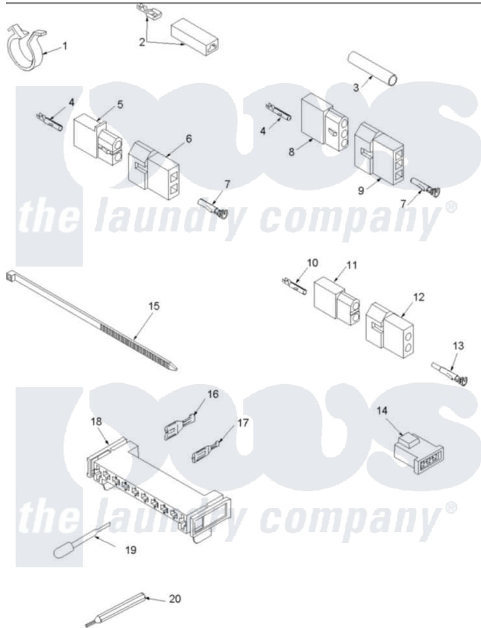
Amana Residential Amana LGD57AW (BOM: PLGD57AW) Dryer Parts Parts Diagram 10 - TERMINALS AND MOTOR CONNECTION BLOCK
