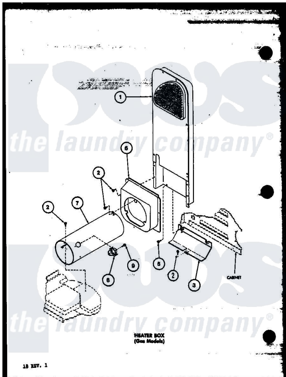
Amana Residential Amana LGD912 (BOM: P7804820W W) Dryer Parts Parts Diagram 04 - HEATER BOX (GAS MODELS)
