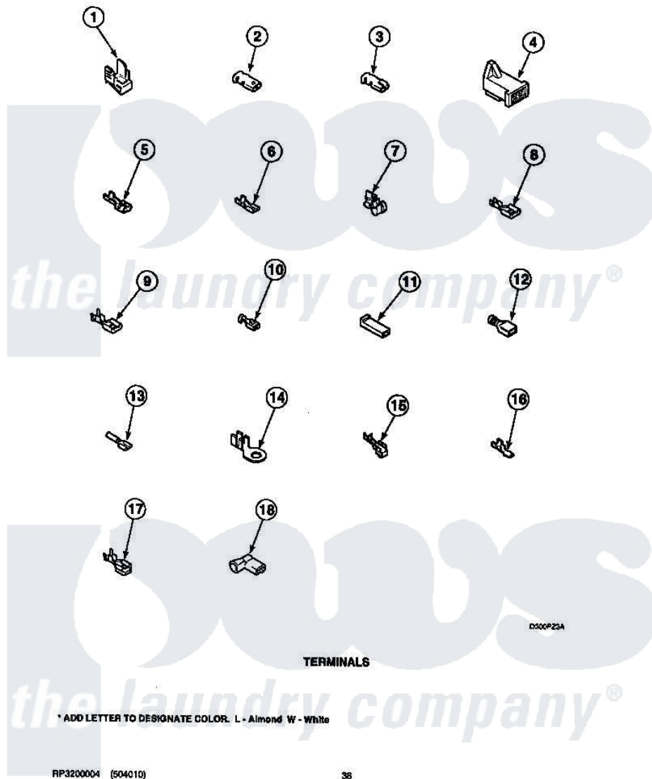
Amana Residential Amana LGS19AW (BOM: PLGS19AW) Dryer Parts Parts Diagram 16 - TERMINALS Click on the part number to view part
