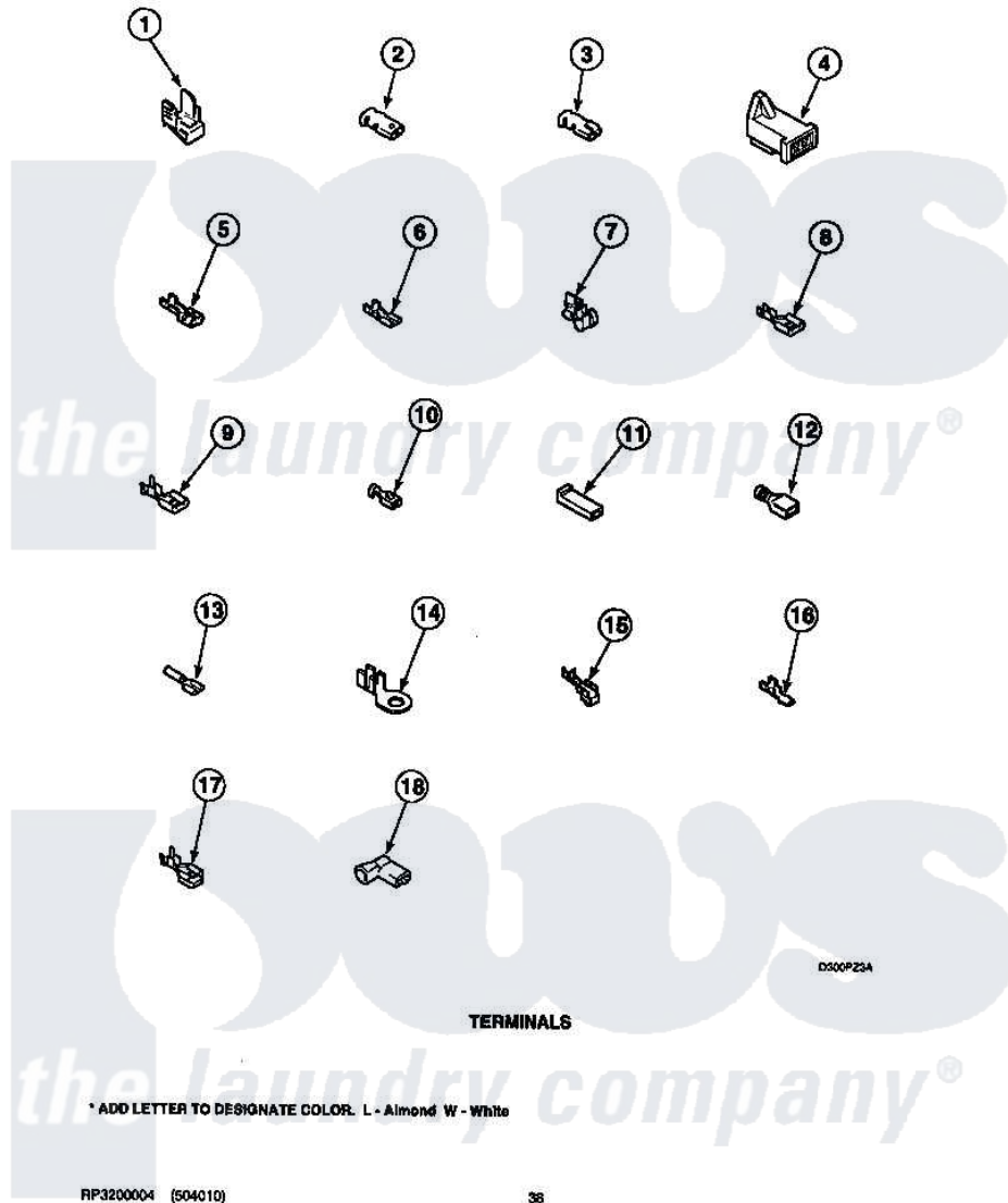
Amana Residential Amana LGS33AW (BOM: PLGS33AW) Dryer Parts Parts Diagram 16 - TERMINALS
