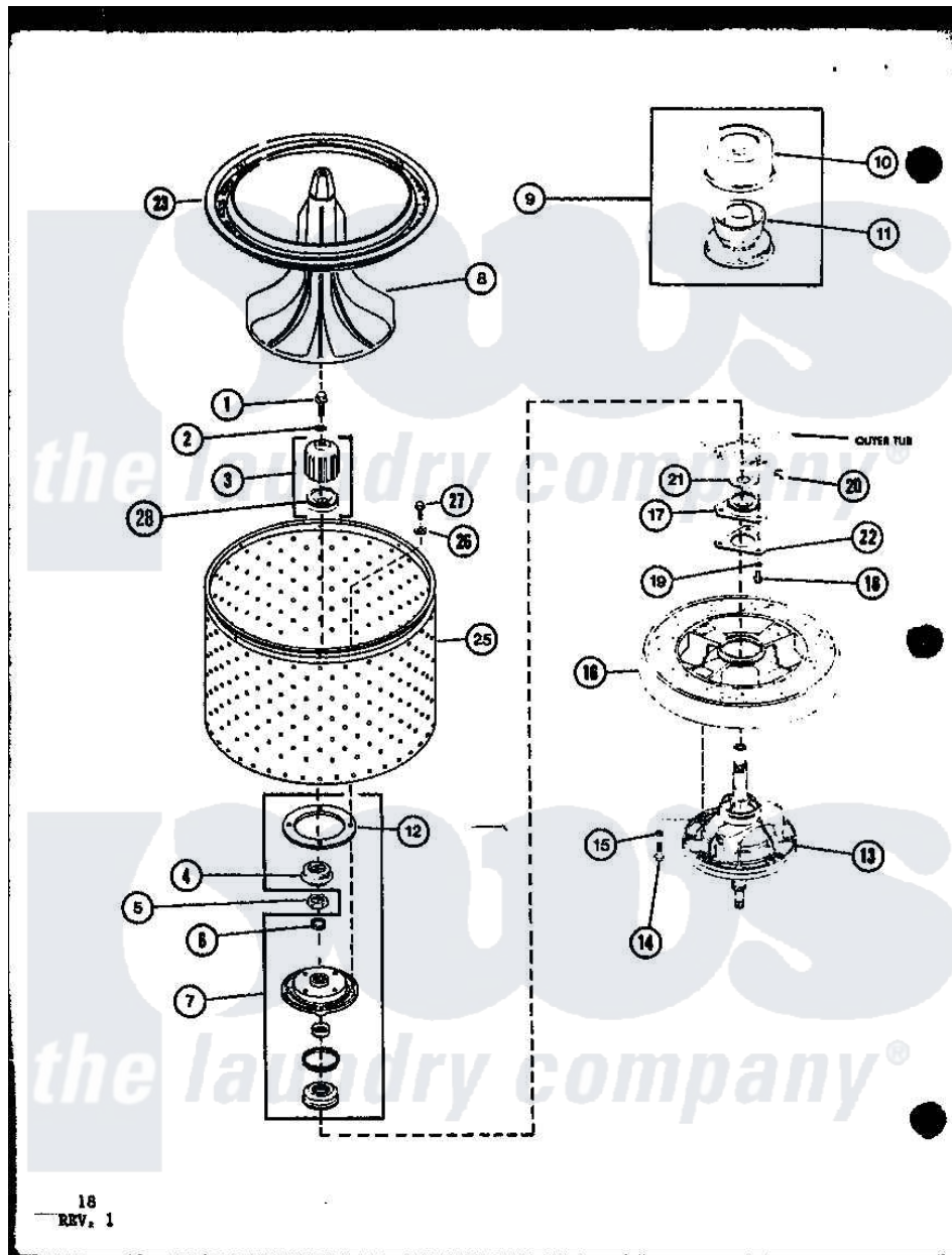
Amana Residential Amana LW1200 (BOM: P7762101W W) Washer Parts Diagram 06 - Page 7 Click on the part number to view part
