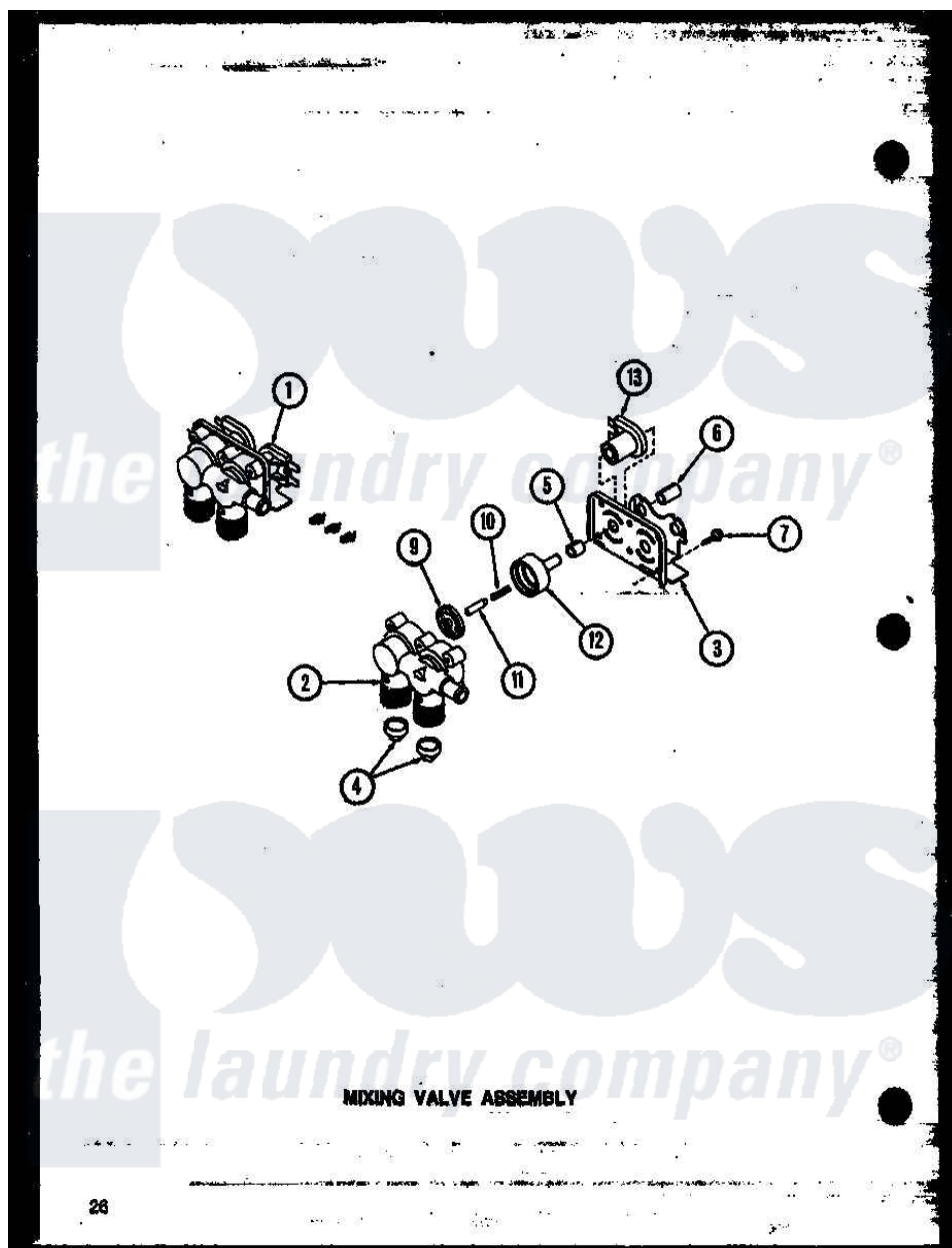
Amana Residential Amana LW2201G (BOM: P1164302W G) Washer Parts Parts Diagram 03 - MIXING VALVE ASSY
