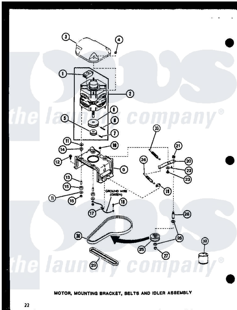
Amana Residential Amana LW2302 (BOM: P1110514W W) Washer Parts Parts Diagram 04 - MOTOR Click on the part number to view part
