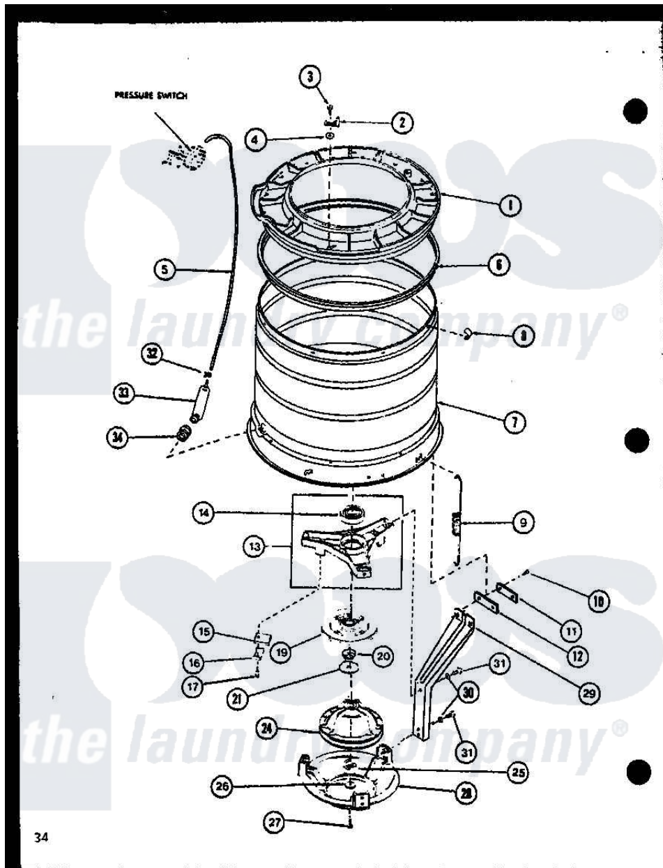
Amana Residential Amana LW2303 (BOM: P1110515W W) Washer Parts Diagram 07 - Page 15 Click on the part number to view part
