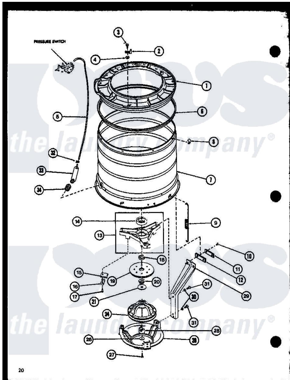
Amana Residential Amana LW2400 (BOM: P7762103W W) Washer Parts Diagram 07 - Page 8 Click on the part number to view part
