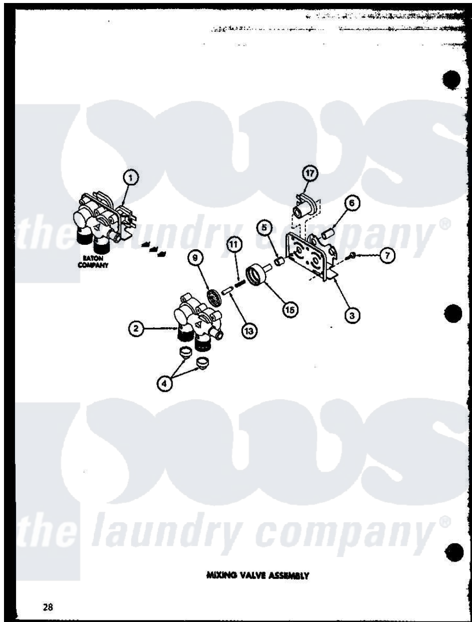
Amana Residential Amana LW2402 (BOM: P7762113W W) Washer Parts Parts Diagram 03 - MIXING VALVE ASSY
