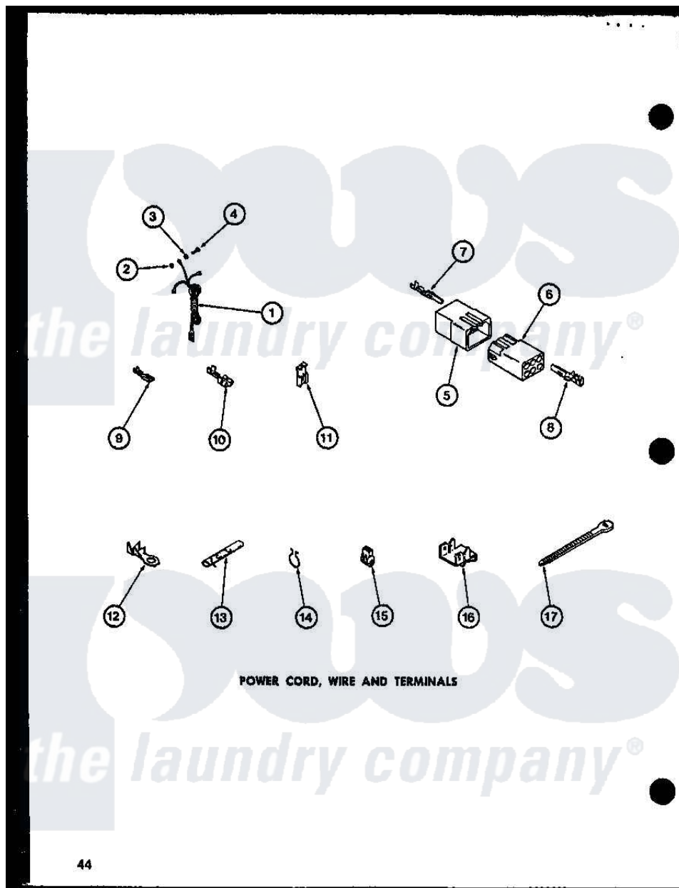
Amana Residential Amana LW2402 (BOM: P7762113W W) Washer Parts Parts Diagram 08 - POWER CORD Click on the part number to view part
