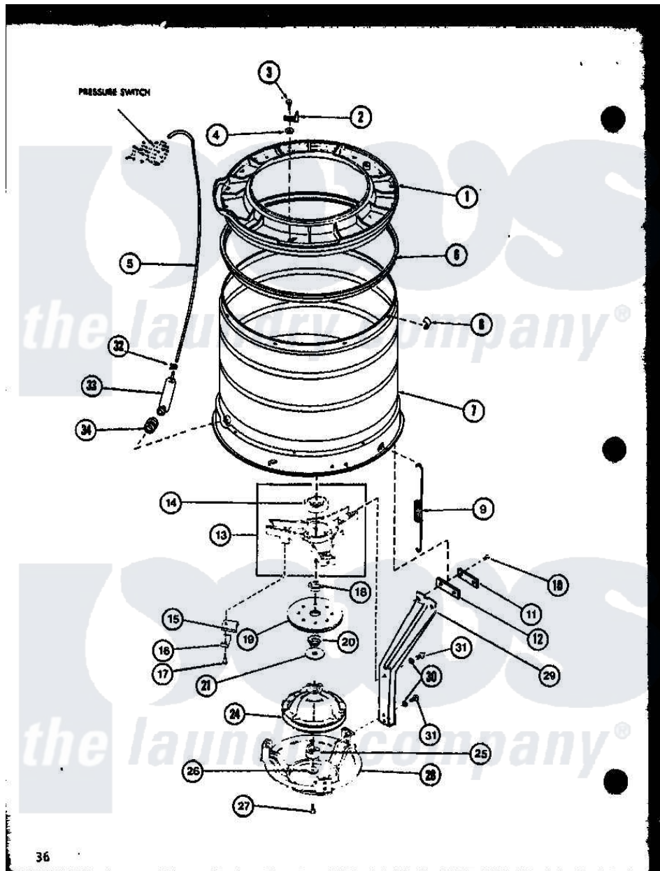
Amana Residential Amana LW2402 (BOM: P7762126W W) Washer Parts Parts Diagram 06 - Page 16 Click on the part number to view part
