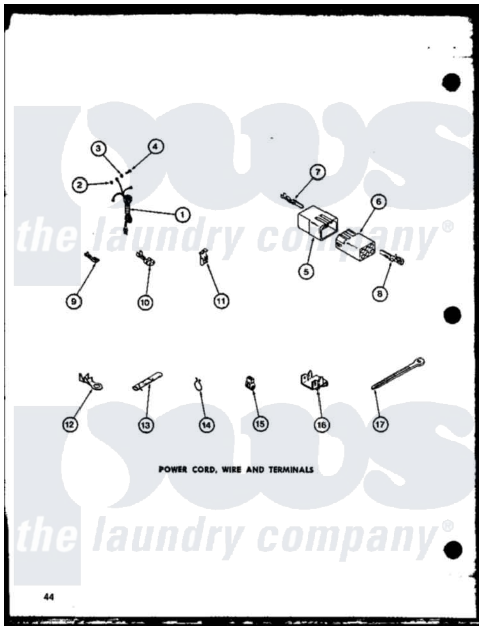
Amana Residential Amana LW2402 (BOM: P7762126W W) Washer Parts Parts Diagram 08 - POWER CORD Click on the part number to view part
