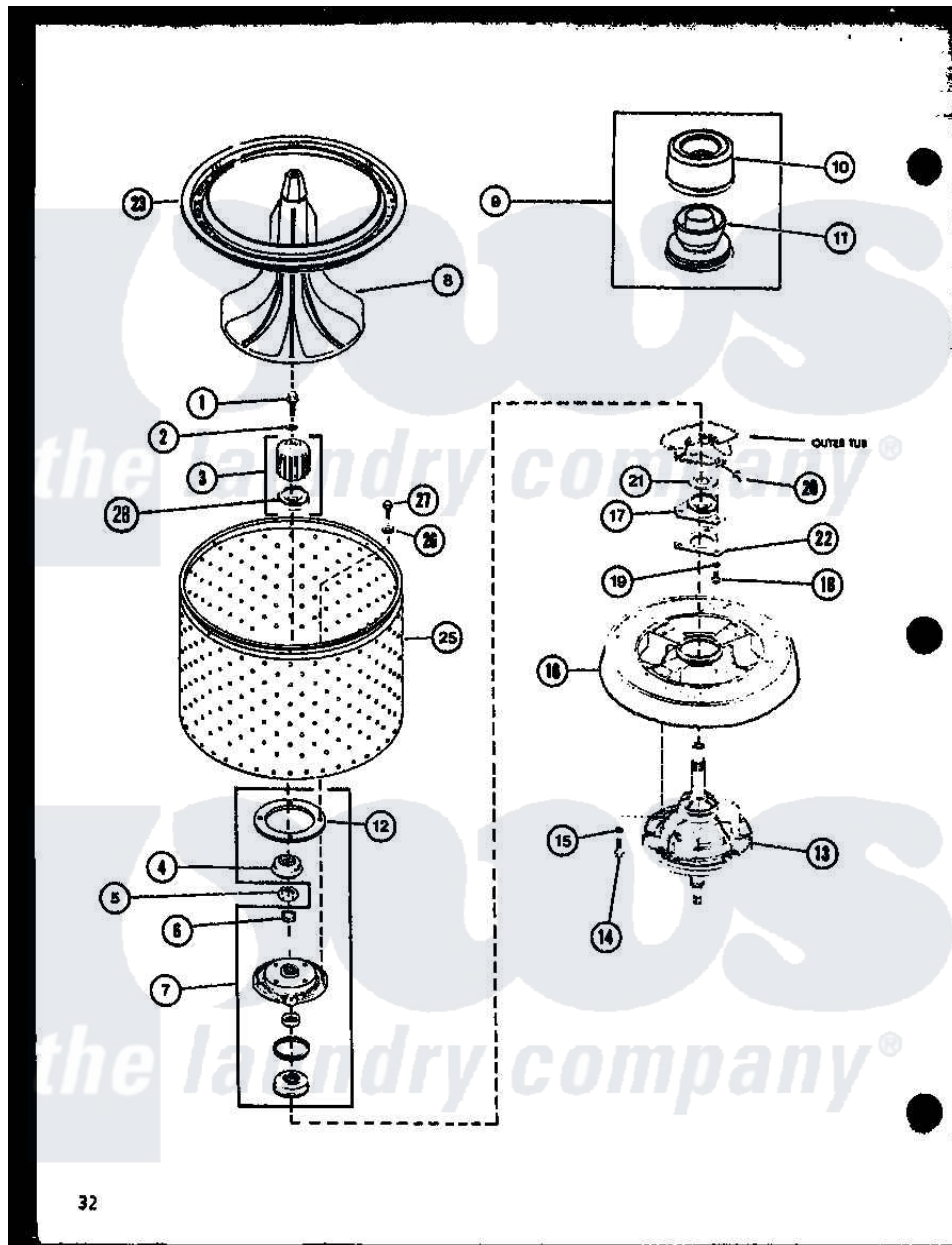
Amana Residential Amana LW2403 (BOM: P7762120W W) Washer Parts Parts Diagram 05 - Page 14 Click on the part number to view part
