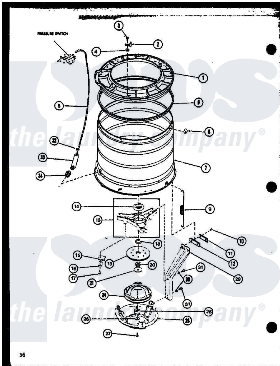
Amana Residential Amana LW2403 (BOM: P7762120W W) Washer Parts Parts Diagram 06 - Page 16 Click on the part number to view part
