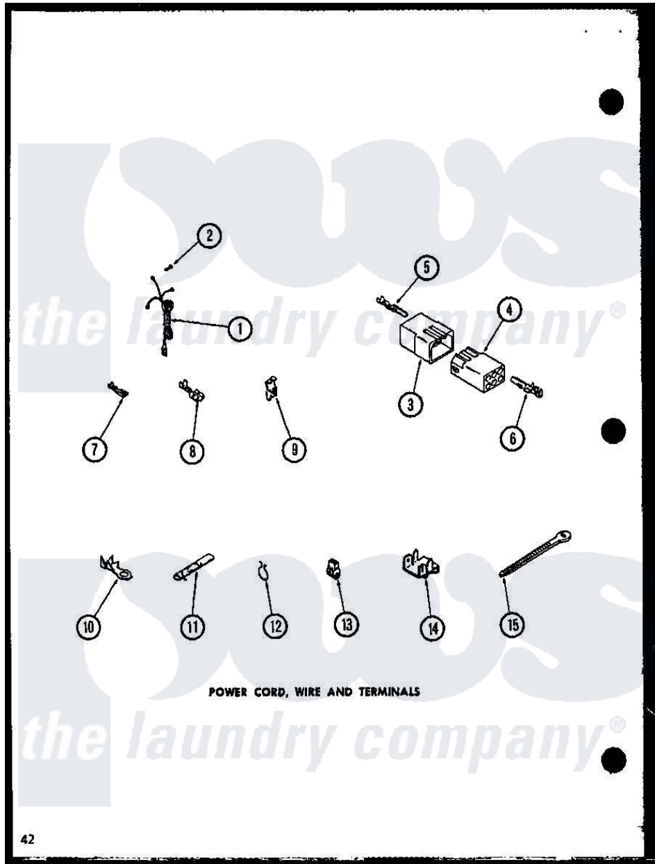
Amana Residential Amana LW2501G (BOM: P1118405W G) Washer Parts Parts Diagram 09 - POWER CORD Click on the part number to view part
