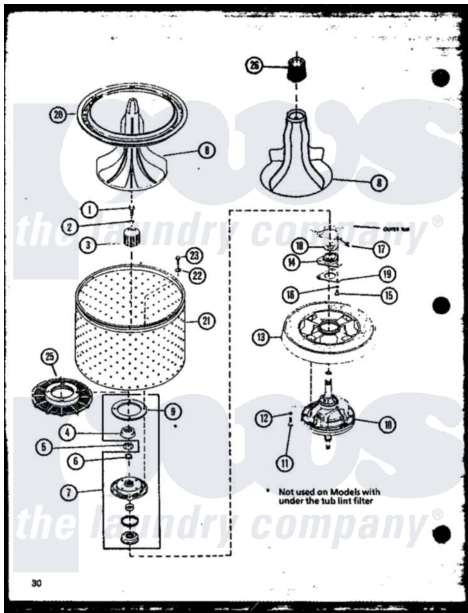
Amana Residential Amana LW2501G (BOM: P1164305W G) Washer Parts Diagram 05 - Page 14 Click on the part number to view part
