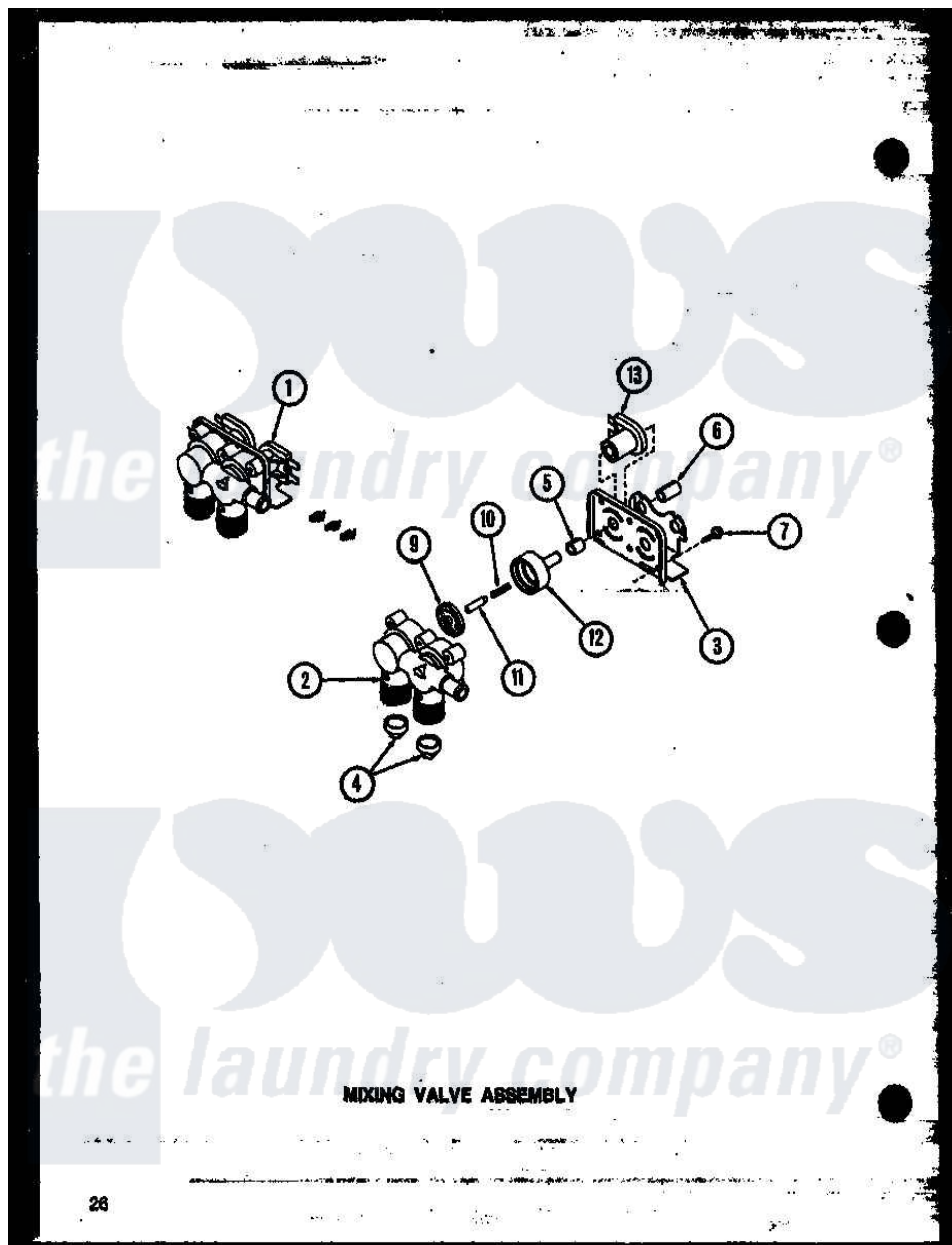
Amana Residential Amana LW2501W (BOM: P1164304W W) Washer Parts Parts Diagram 03 - MIXING VALVE ASSY
