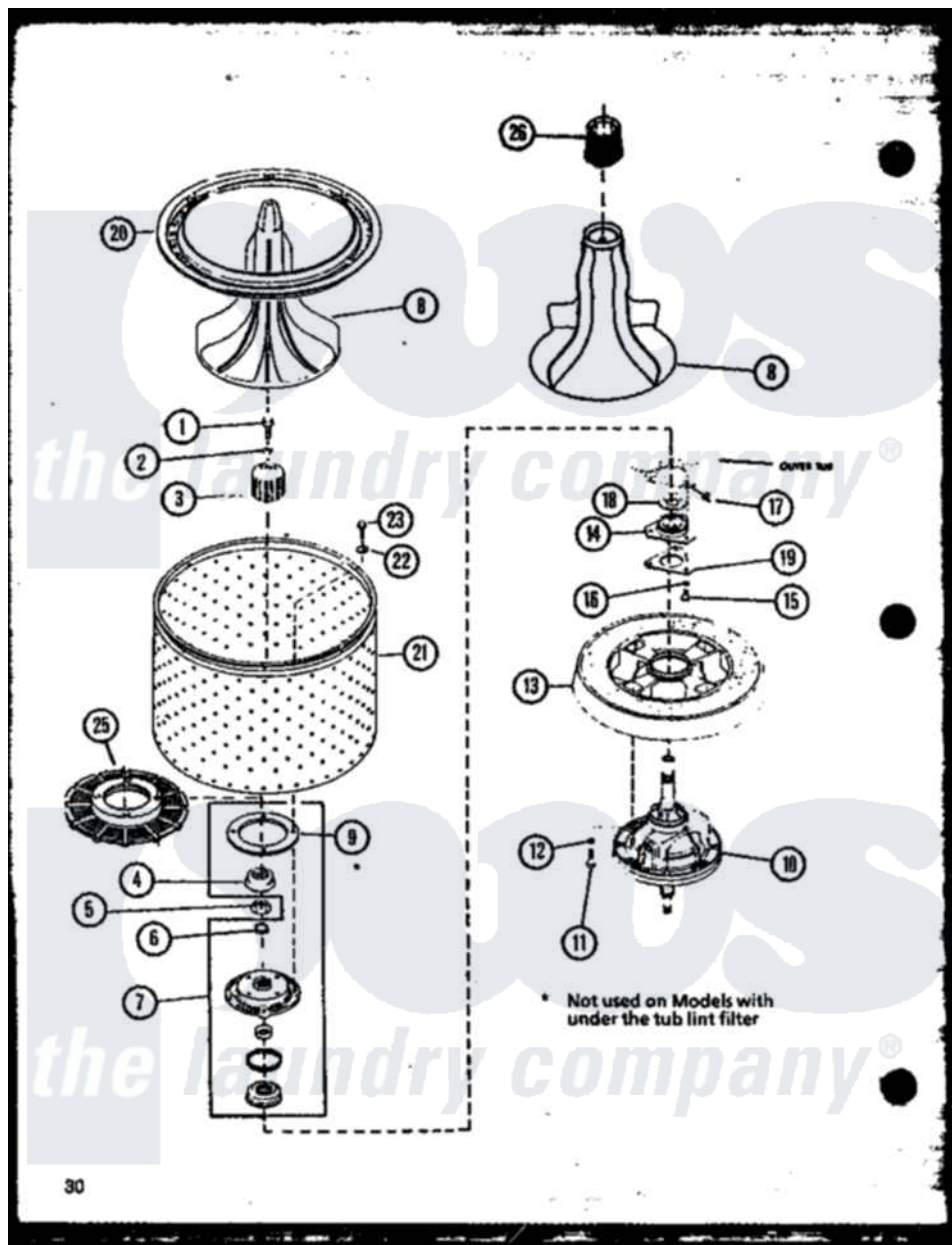
Amana Residential Amana LW2501W (BOM: P1164304W W) Washer Parts Parts Diagram 05 - Page 14
