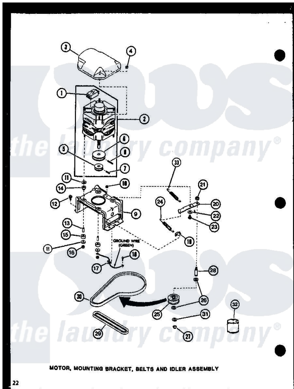
Amana Residential Amana LW2503L (BOM: P1118412W L) Washer Parts Parts Diagram 04 - MOTOR Click on the part number to view part
