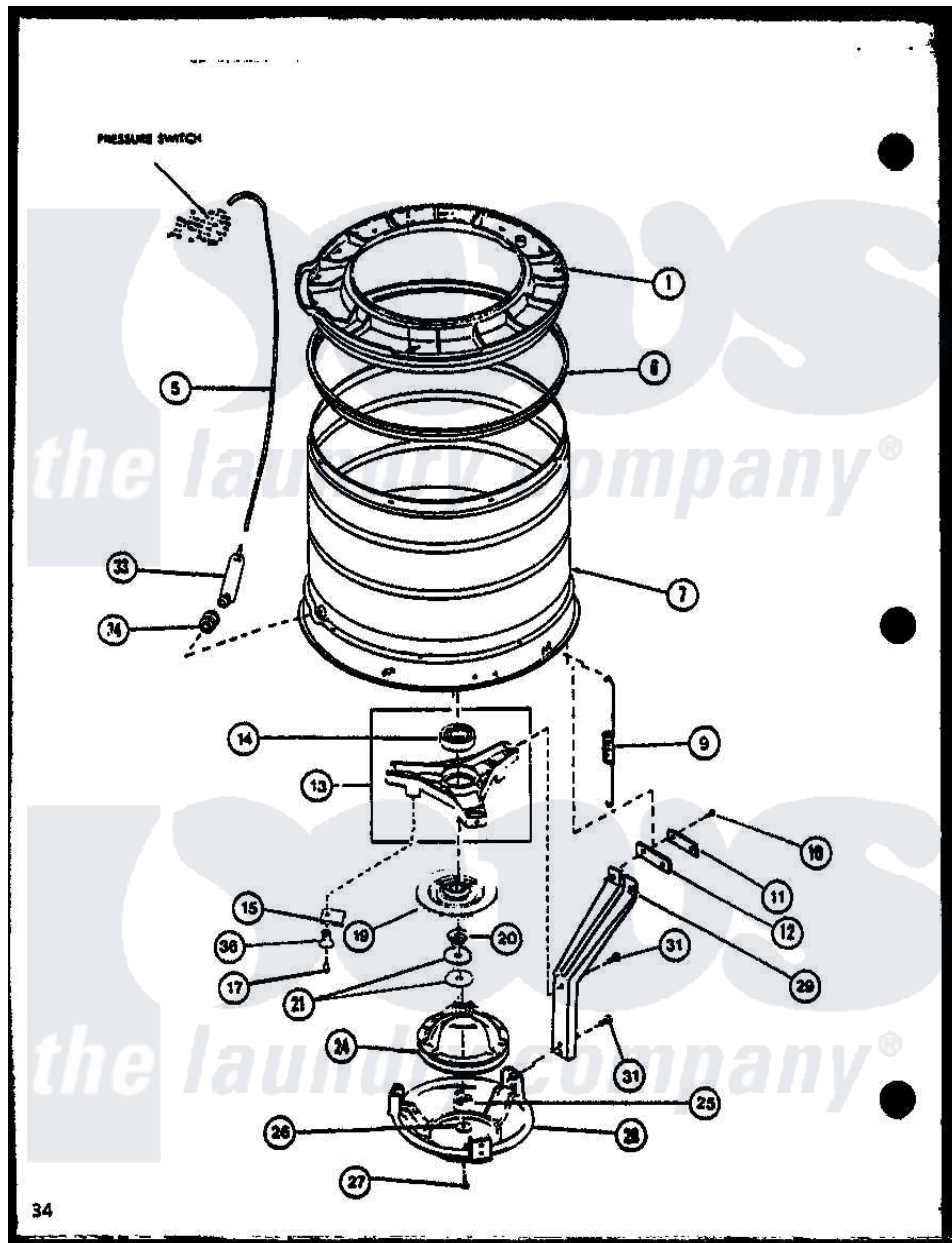
Amana Residential Amana LW2503L (BOM: P1118412W L) Washer Parts Diagram 07 - Page 15 Click on the part number to view part
