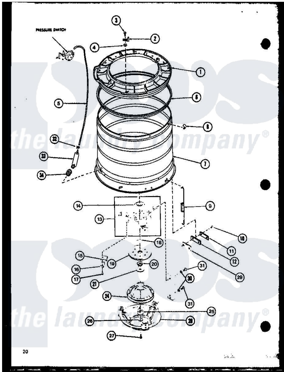
Amana Residential Amana LW2600 (BOM: P7804701W W) Washer Parts Parts Diagram 07 - Page 8 Click on the part number to view part
