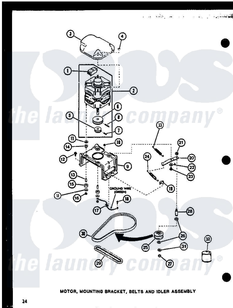
Amana Residential Amana LW3403W (BOM: P1118419W W) Washer Parts Parts Diagram 04 - MOTOR Click on the part number to view part
