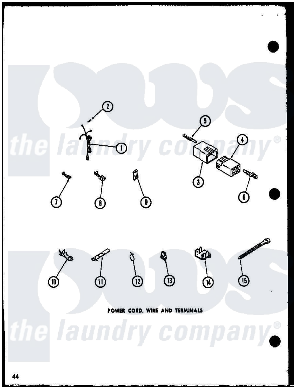
Amana Residential Amana LW3403W (BOM: P1118419W W) Washer Parts Parts Diagram 09 - POWER CORD Click on the part number to view part
