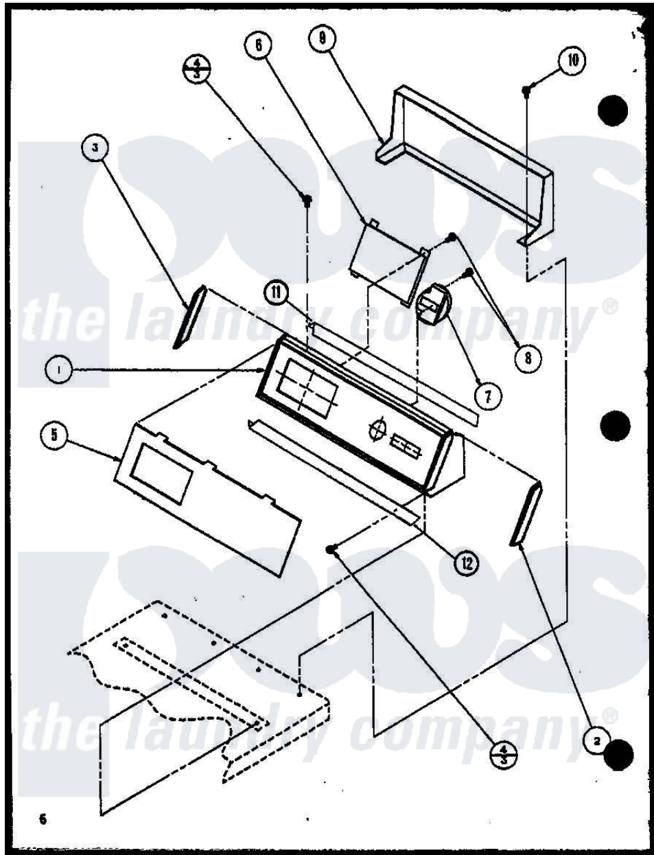
Amana Residential Amana LW3603 (BOM: P1110506W W) Washer Parts Diagram 05 - Page 1 Click on the part number to view part
