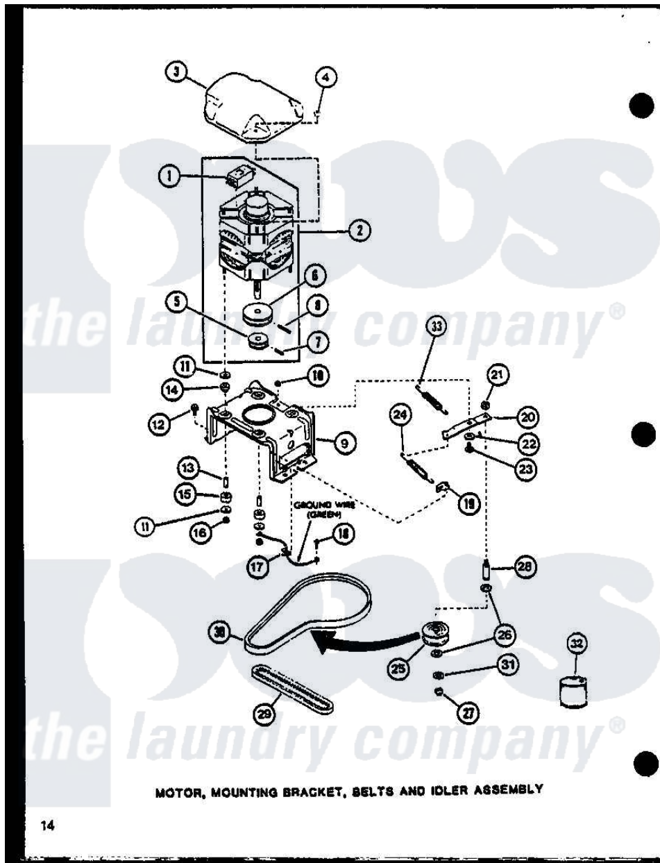
Amana Residential Amana LW3903L (BOM: P1122404W L) Washer Parts Parts Diagram 04 - MOTOR Click on the part number to view part
