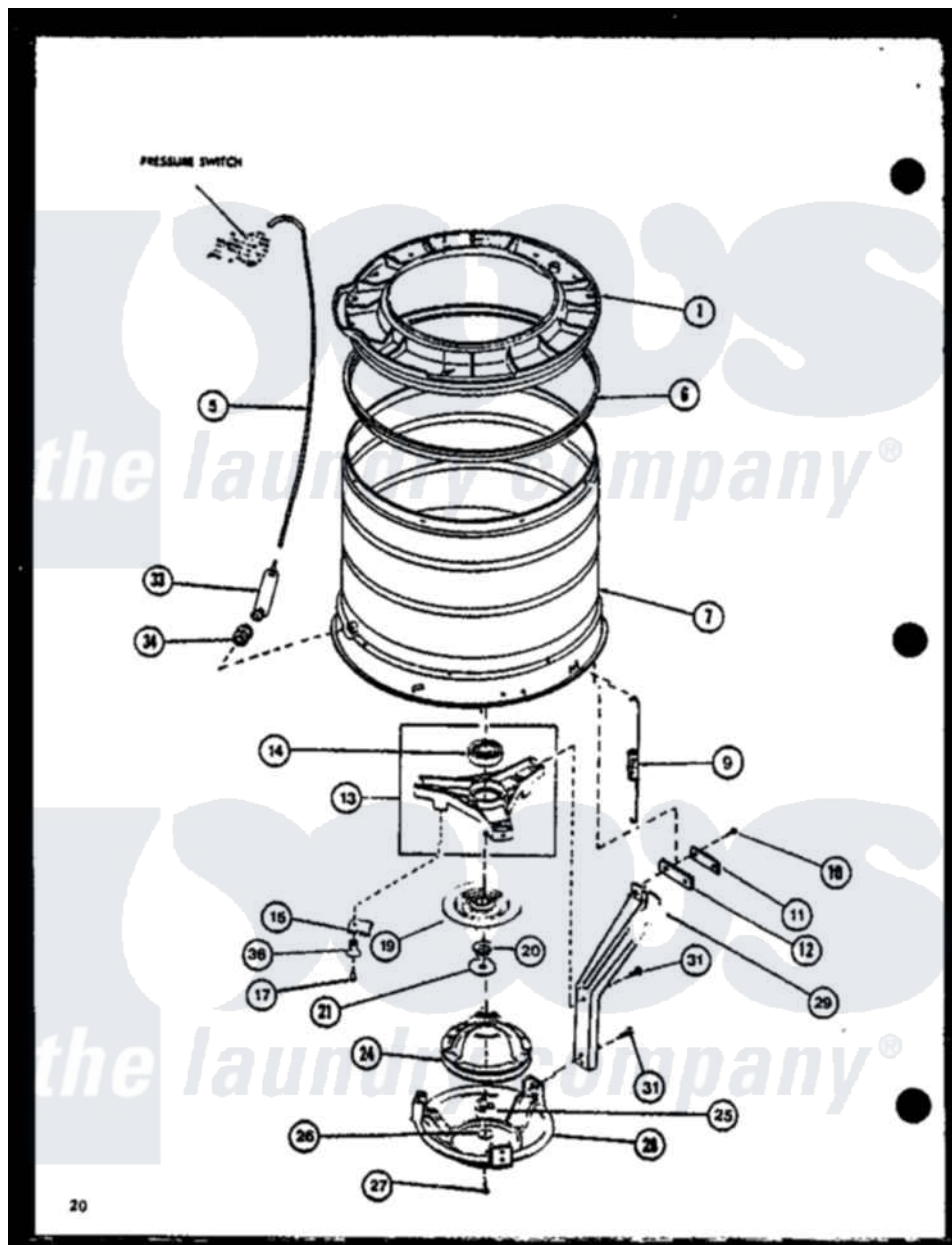
Amana Residential Amana LW3903L (BOM: P1122404W L) Washer Parts Parts Diagram 06 - Page 8 Click on the part number to view part
