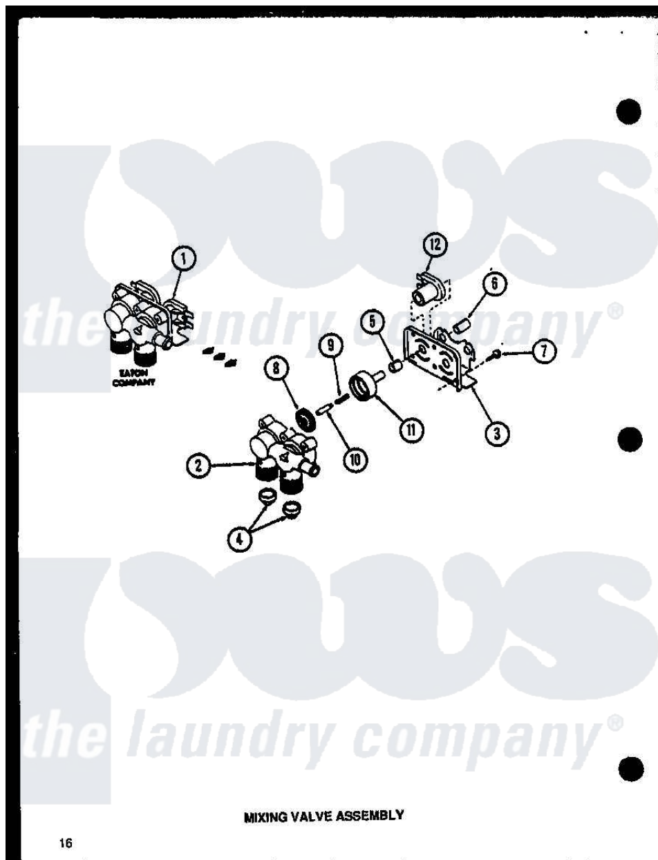
Amana Residential Amana LW3903W (BOM: P1122407W W) Washer Parts Parts Diagram 04 - MIXING VALVE ASSY Click on the part number to view part
