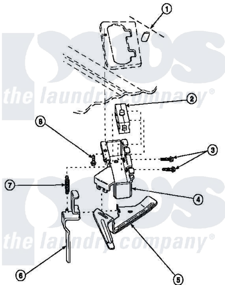
Amana Residential Amana LW6661W2 (BOM: PLW6661W2 B) Washer Parts Parts Diagram 15 - OUT-OF-BALANCE SWITCH
