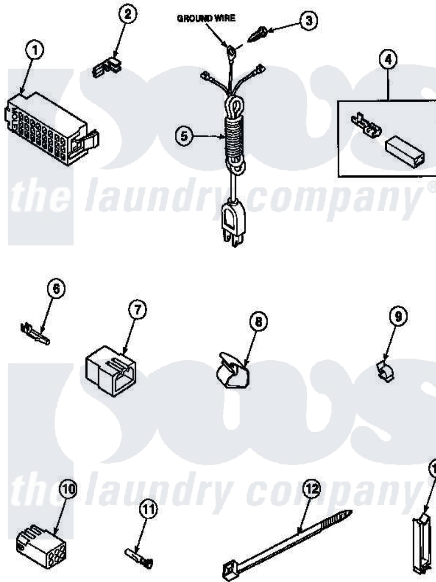
Amana Residential Amana LW7563W2 (BOM: PLW7563W2 B) Washer Parts Parts Diagram 16 - POWER CORD AND TERMINALS
