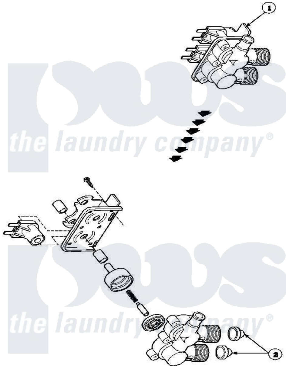
Amana Residential Amana LW8203W2B (BOM: PLW8203W2 A) Washer Parts Parts Diagram 18 - MIXING VALVE
