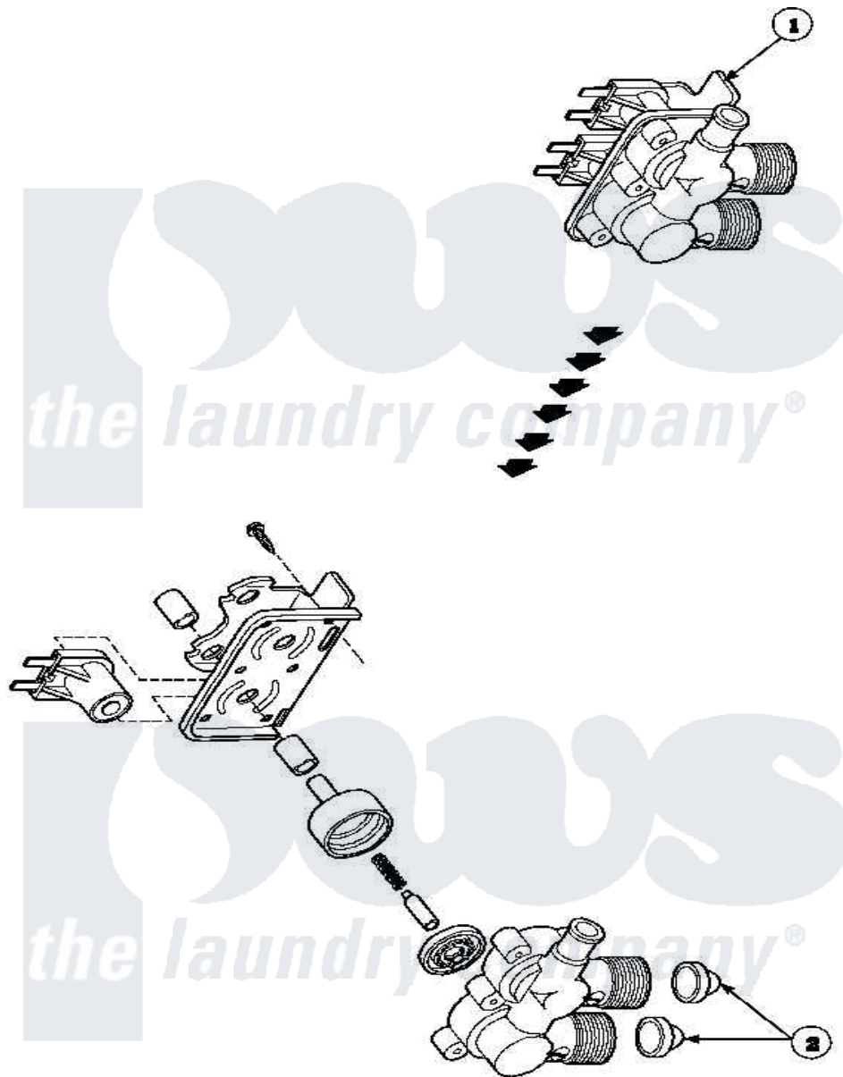
Amana Residential Amana LW8413L2 (BOM: PLW8413L2 A) Washer Parts Parts Diagram 18 - MIXING VALVE Click on the part number to view part
