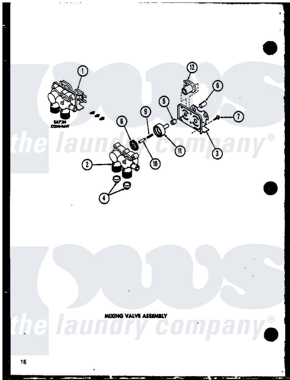
Amana Residential Amana LW9003 (BOM: P1110503W W) Washer Parts Parts Diagram 03 - MIXING VALVE ASSY
