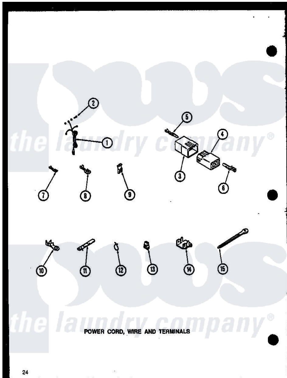
Amana Residential Amana LW9103W (BOM: P1122812W W) Washer Parts Parts Diagram 08 - POWER CORD Click on the part number to view part
